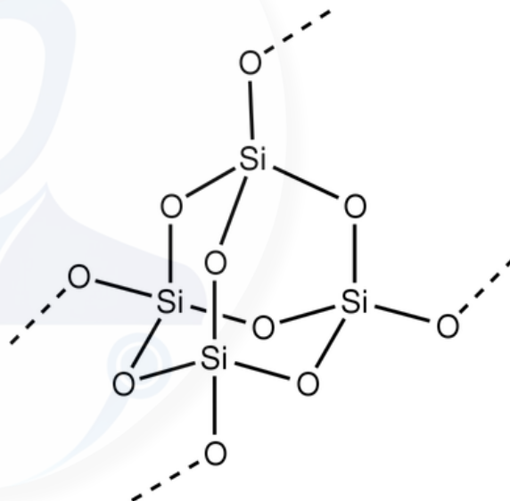
Silicon dioxide
