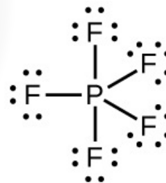
PF 5
