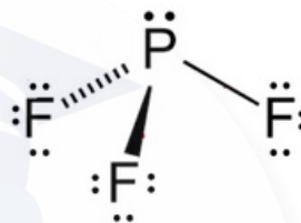
(PF 3 )
