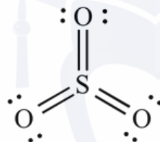
Sulfur trioxide
